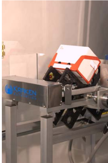
Star-Wheel Carton Turner
