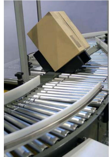
Star-Wheel Case Turner
